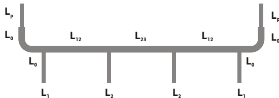
Microstrip Line High Pass Filter Circuit
